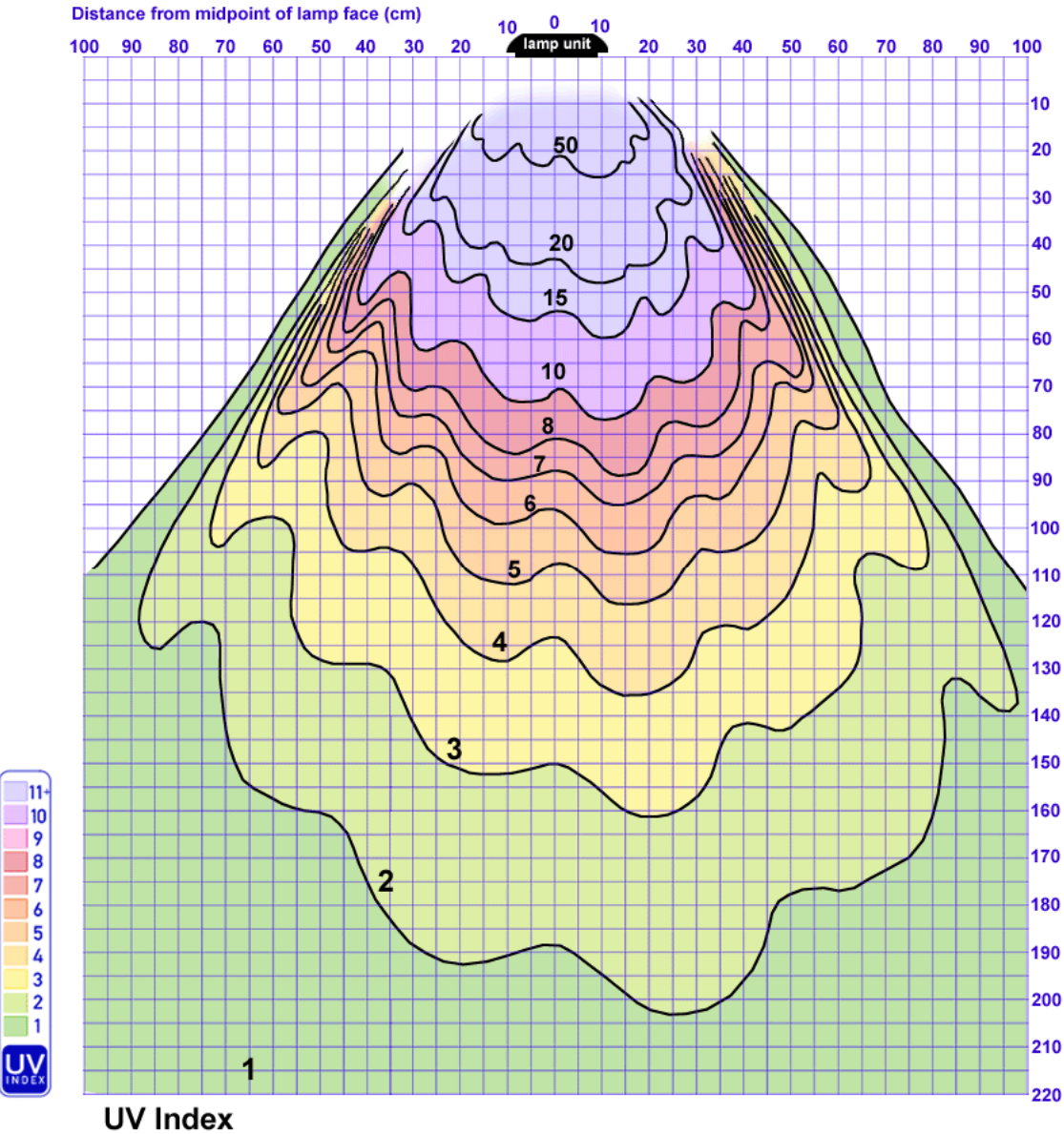
UV Index iso-irradiance diagram (spread pattern) of lamp ref. BLIH1 tested 15.06.2016 after 105hrs burn
